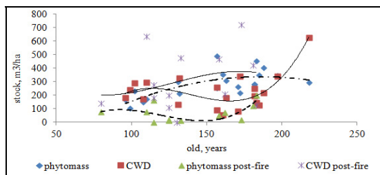
Fig. 7. Dynamics of phytomass and phytodetritus stocks in disturbed and undisturbed dark coniferous forests
