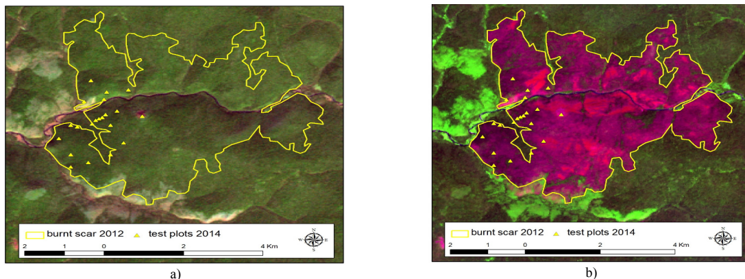
Fig. 4. Area burnt in 2012 located near Kutukas river: a) Landsat 5, September 13, 2011; b) Landsat 8, August 17, 2013
